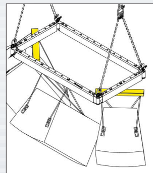
Cross Arms in yellow
