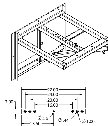
Cross Arm
