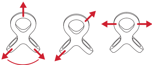
NFPA General Use Configuration MBS 45 kN (10,116 LBF)
